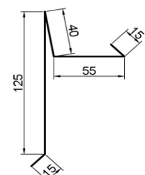
12. Ortgang Standard 25
